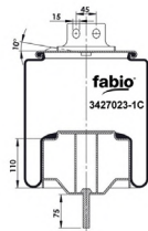
CROSS SECTION
