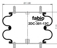
CROSS SECTION
