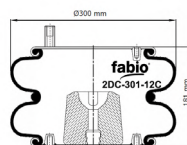
CROSS SECTION
