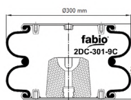
CROSS SECTION
