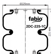
CROSS SECTION
