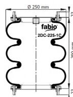
CROSS SECTION
