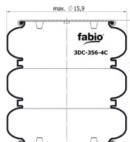
CROSS SECTION
