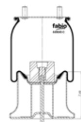
CROSS SECTION
