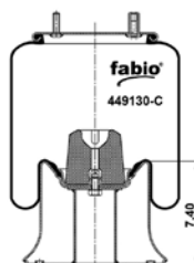
CROSS SECTION
