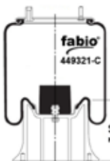
CROSS SECTION
