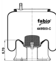
CROSS SECTION
