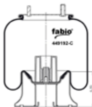
CROSS SECTION
