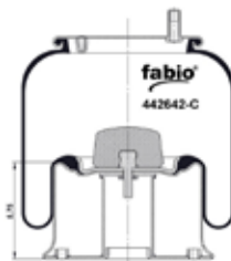
CROSS SECTION
