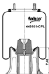
CROSS SECTION
