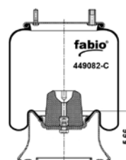
CROSS SECTION
