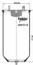
CROSS SECTION
