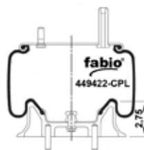
CROSS SECTION
