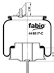
CROSS SECTION
