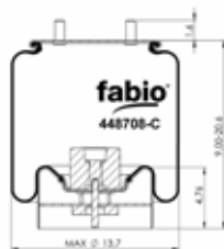
CROSS SECTION
