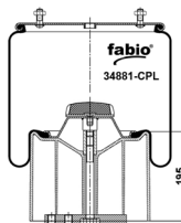
CROSS SECTION
