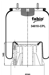
CROSS SECTION
