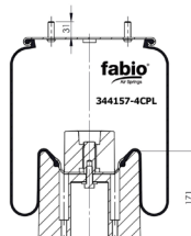
CROSS SECTION
