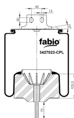
CROSS SECTION
