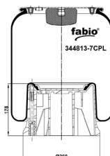
CROSS SECTION
